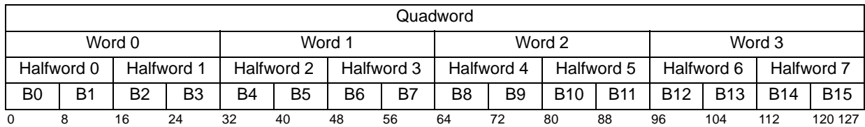
Figure 56. Vector Register elements
