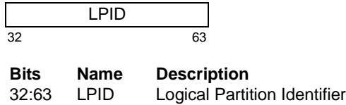
Figure 4. Logical Partition Identification Register
