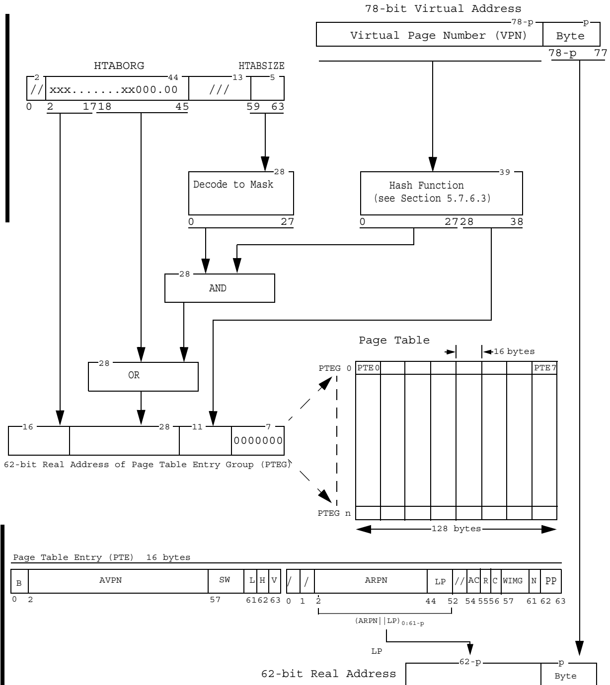
Figure 18. Translation of 78-bit virtual address to 62-bit real address
