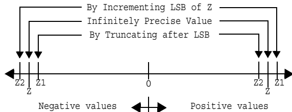
Figure 50. Selection of Z1 and Z2
