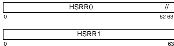
Figure 31. Hypervisor Save/Restore Registers
