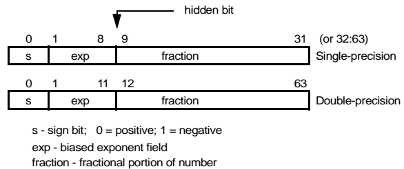
Figure 68. Floating-Point Data Format
